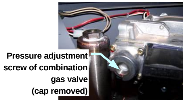
Illustration 3 - Gas Valve Adjustment Screw
