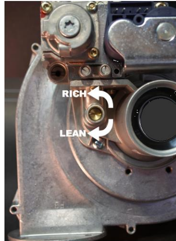
Illustration 2 - Air/Gas Mixture Ratio Screw
